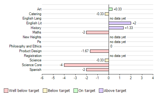
Residuals: Grade
